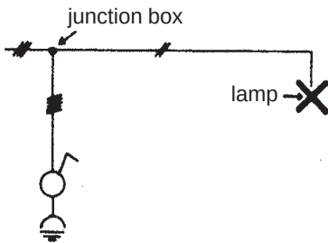
Figure 2. Single-pole representation of the lighting circuit
