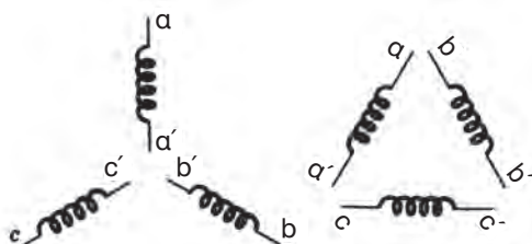
Star (Y) connection Delta ( \Delta ) connection
