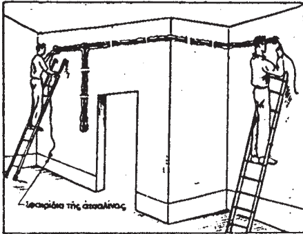
9. Drawing cables and wires along conduits
