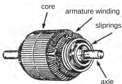
Rotor of an AC generator
