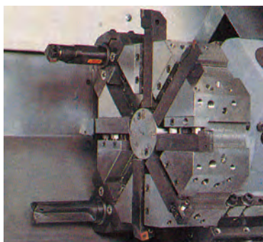
A revolving turret
