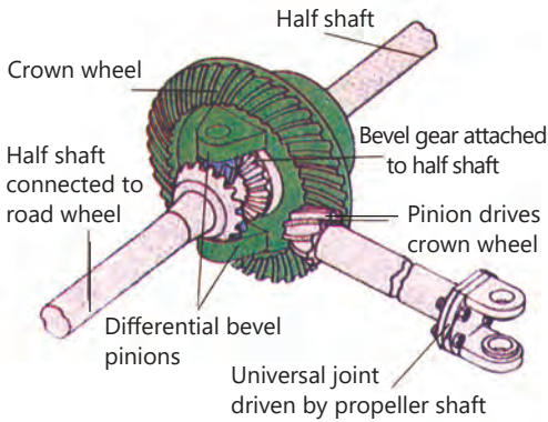
Differential
