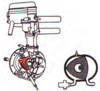
INTERNAL COMBUSTION ROTARY ENGINE (WANKEL)
