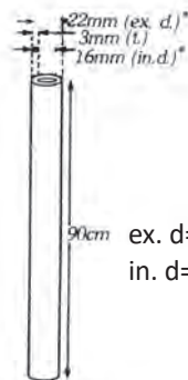
4. Steel tube
