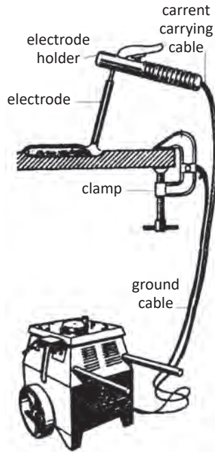
Welding machine
