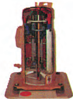
SCROLL COMPRESSOR
