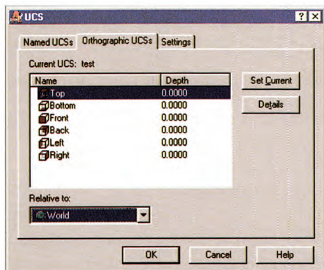
4.5. ORTHOGRAPHIC UCS
