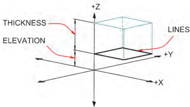
4.7.ELEVATION
