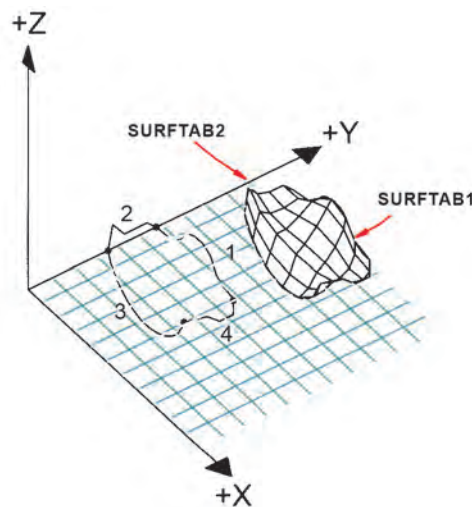
7.9.EDGESURF
