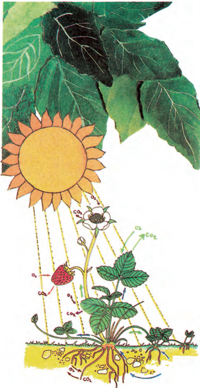
Photosynthesis
