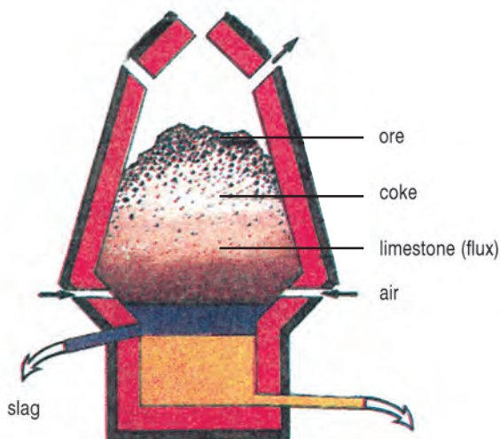
Blast furnace
