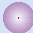
F (72 pm)
