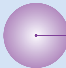
I (133pm)
