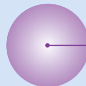
CL (99 pm)
