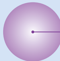
Br (114 pm)
